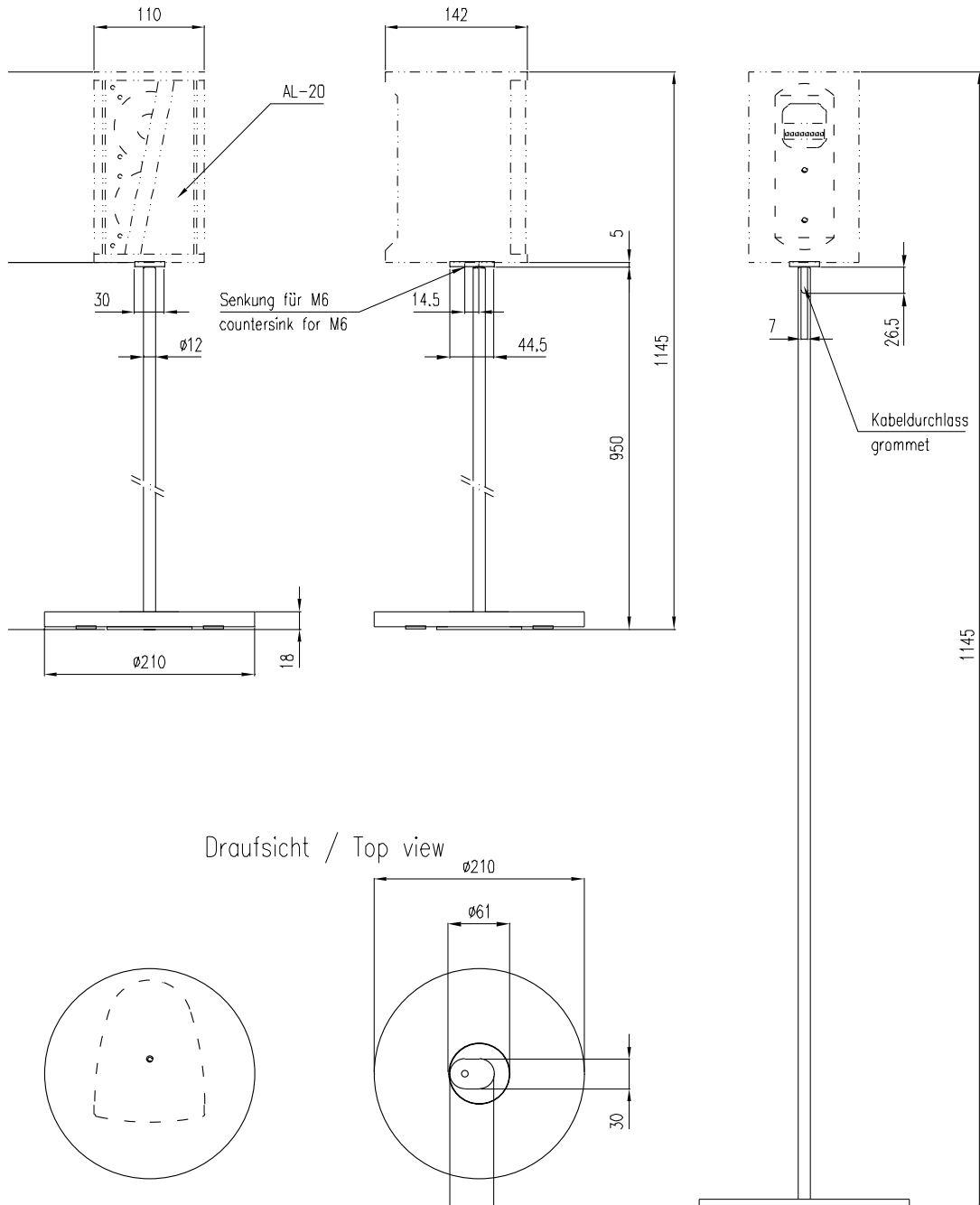
/orderansicht / Front view
