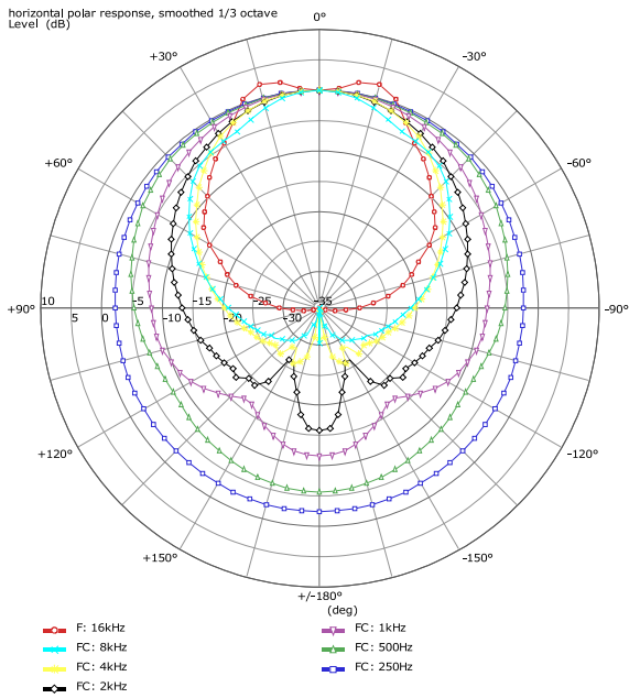
Abbildung 1: AT-061 Horizontal polar response
