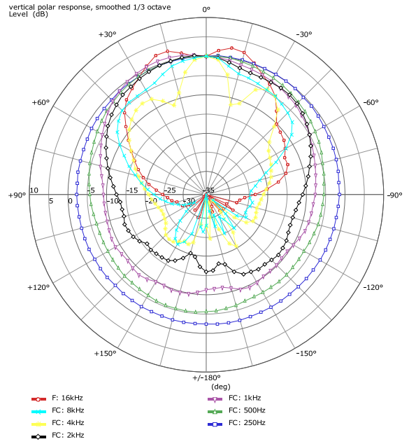
Abbildung 2: AT-061 Vertical polar response
