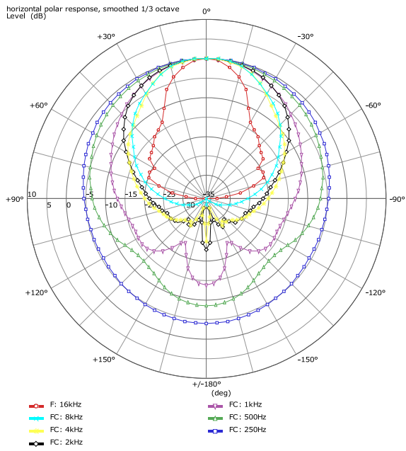
Abbildung 1: AT-221w 60x40 Horizontal polar response
