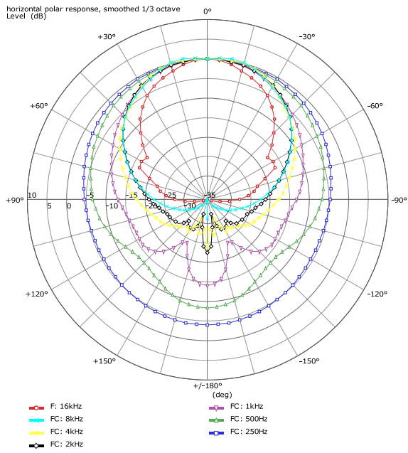
Abbildung 1: AT-221w 90x60 Horizontal polar response
