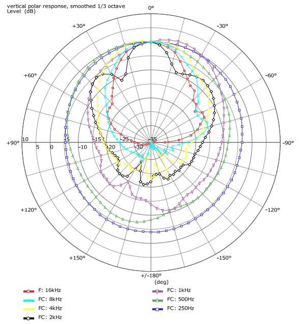
Abbildung 2: AT-221w 90x60 Vertical polar response
