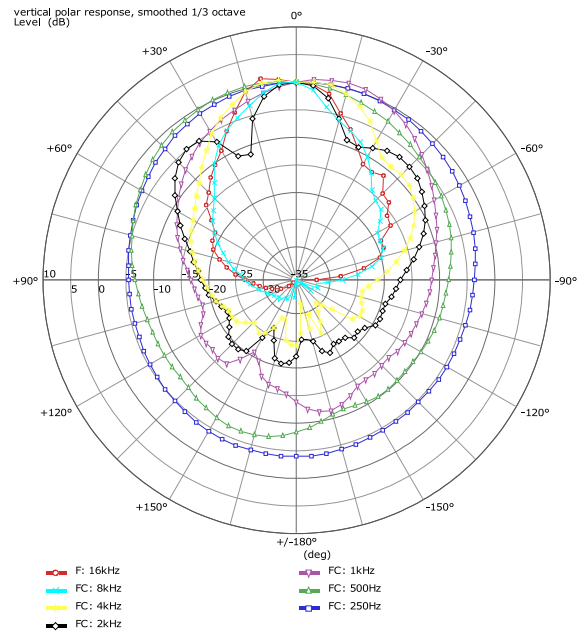
Abbildung 2: AT-221w 60x40 Vertical polar response
