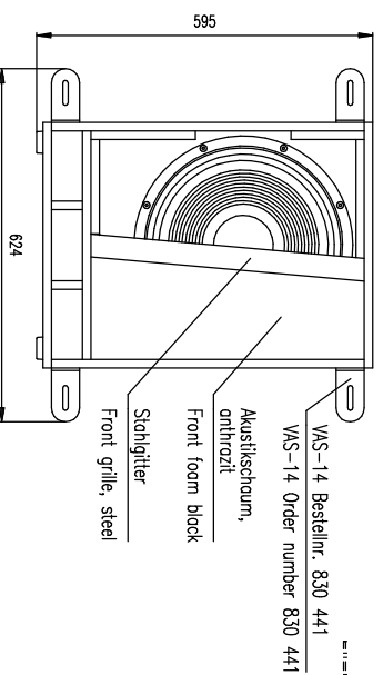
Vorderansicht V. 4 / Front view V. 4
